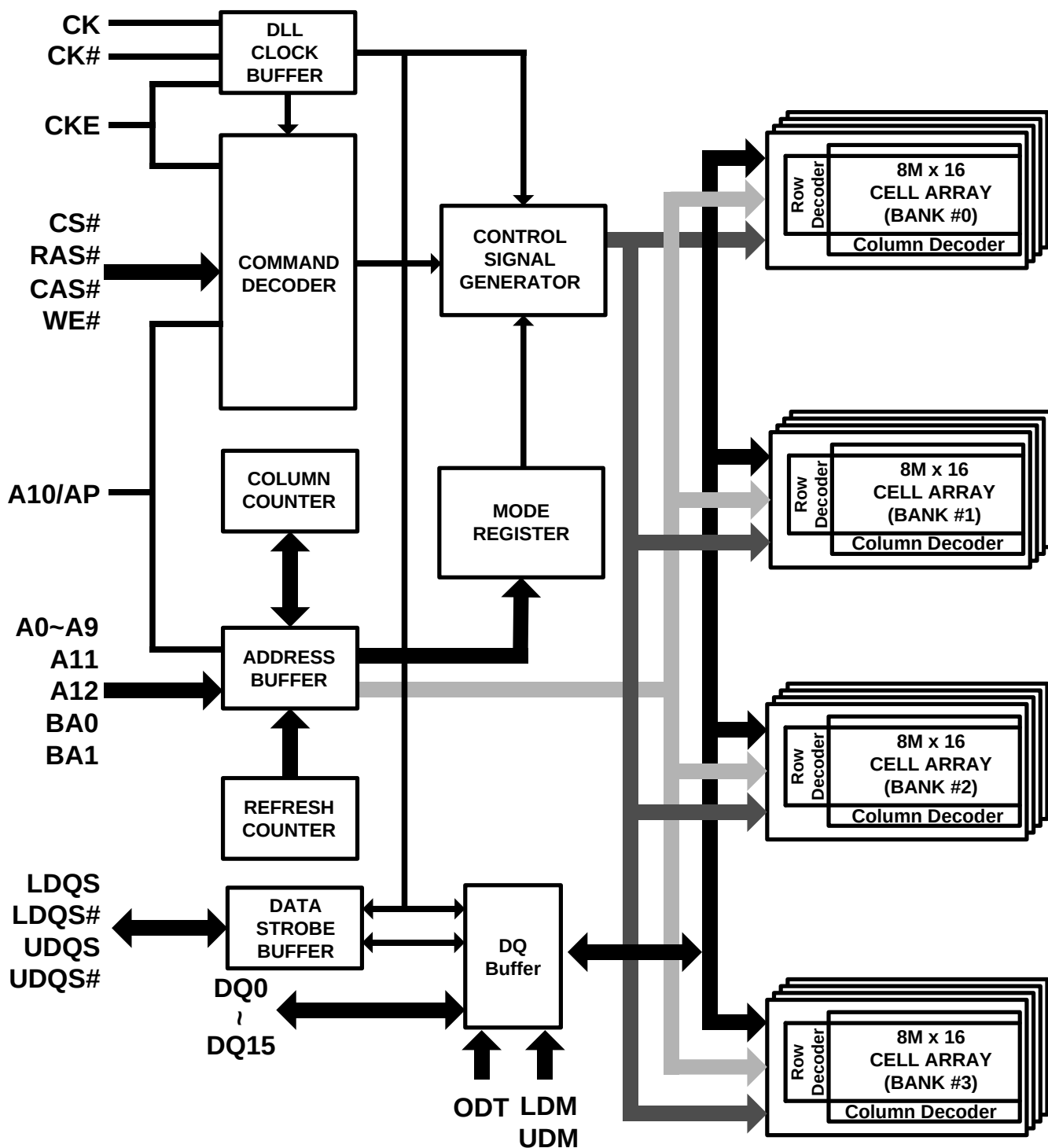
Figure 2. Block Diagram
