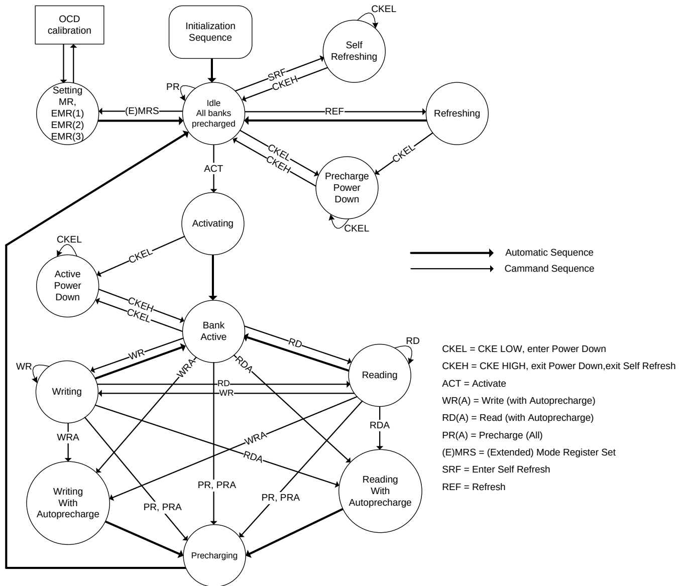
Figure 3. State Diagram
