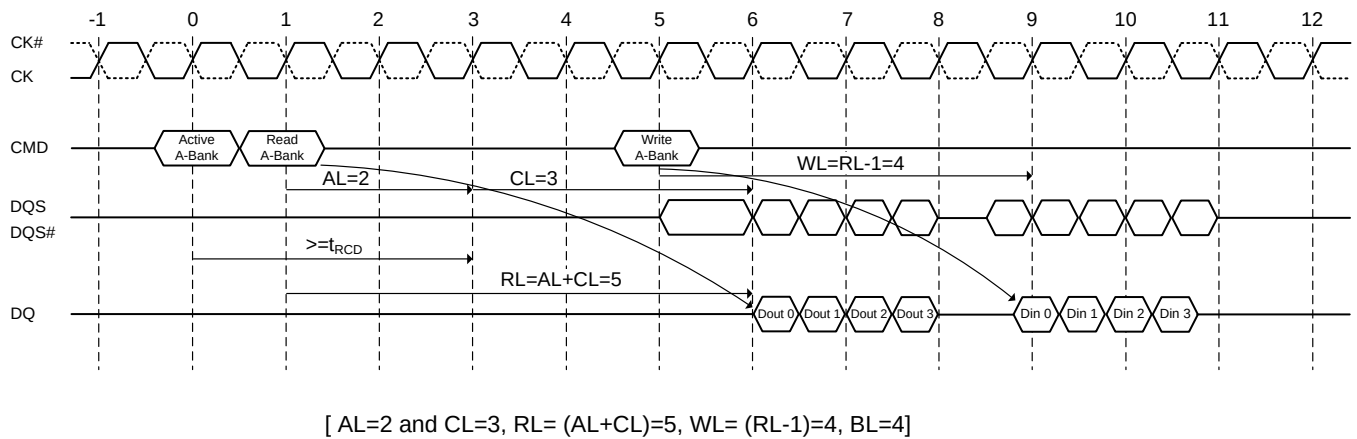
Figure 20. Posted CAS# operation: AL=2, Read followed by a write to the same bank
