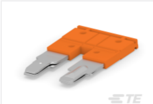
TE Part #1SNK912302R0000 JB12-2
