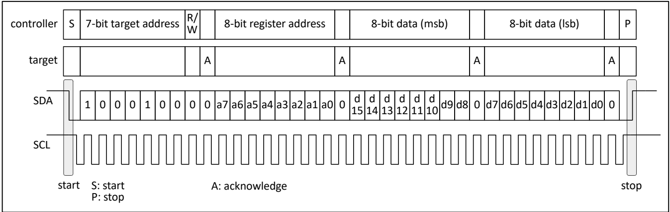
Figure 18: Basic data transfer write sequence with I²C static addressing
