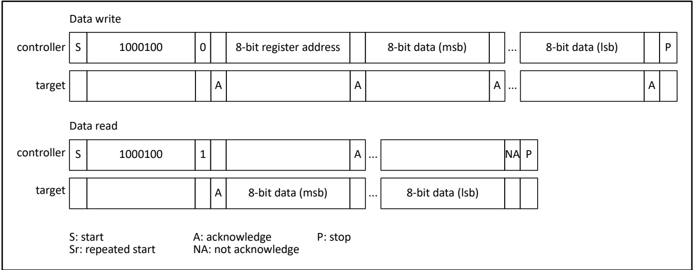
Figure 19: Typical data-transfer sequences with I²C static addressing
