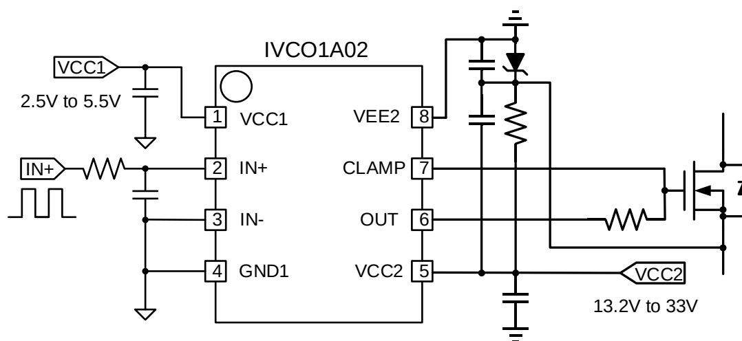
Figure 26. Typical negative bias with Zener diode (IVCO1A02)
