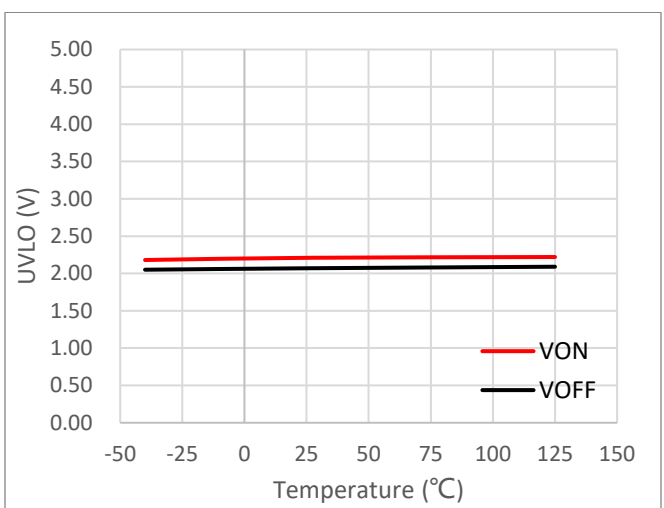
Figure 13. UVLO of VCC1 vs Temperature
