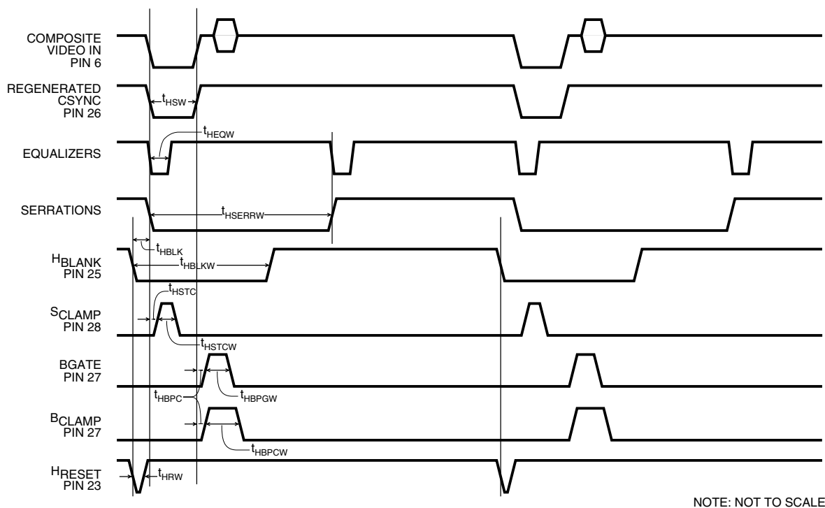
Figure 1. Line Rate Waveforms
