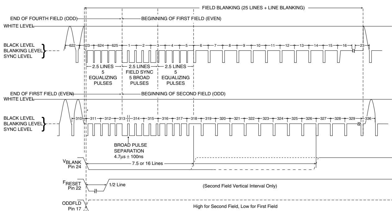
Figure 3. PAL 625 Field Rate Waveforms
