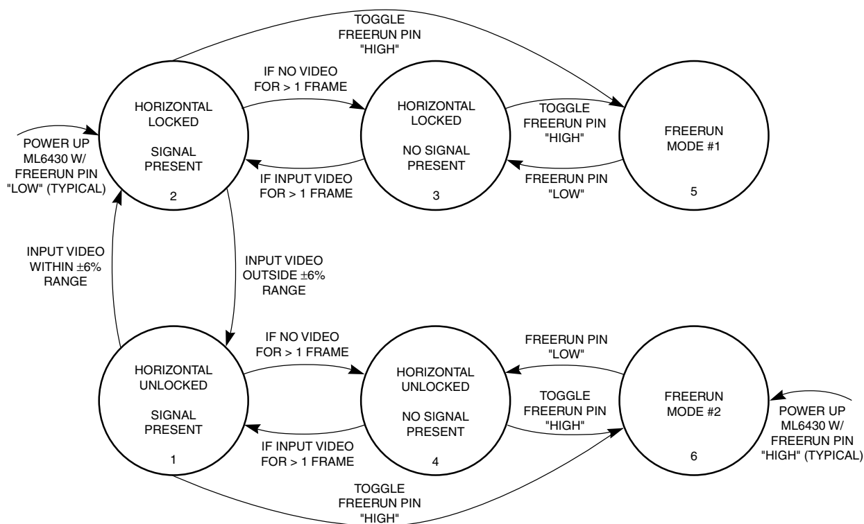
Figure 4. ML6430 Freerun Mode State Diagram
