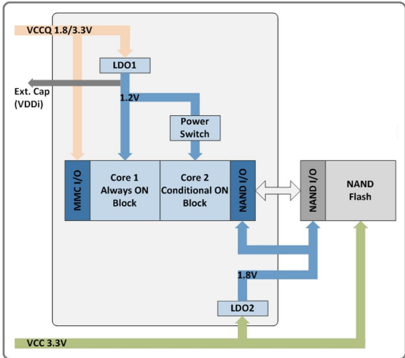
Figure 4. JSMC04AUM1ASAEA-SU Block Diagram
