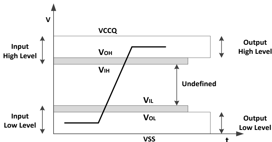
Figure 9. Bus Signal Levels
