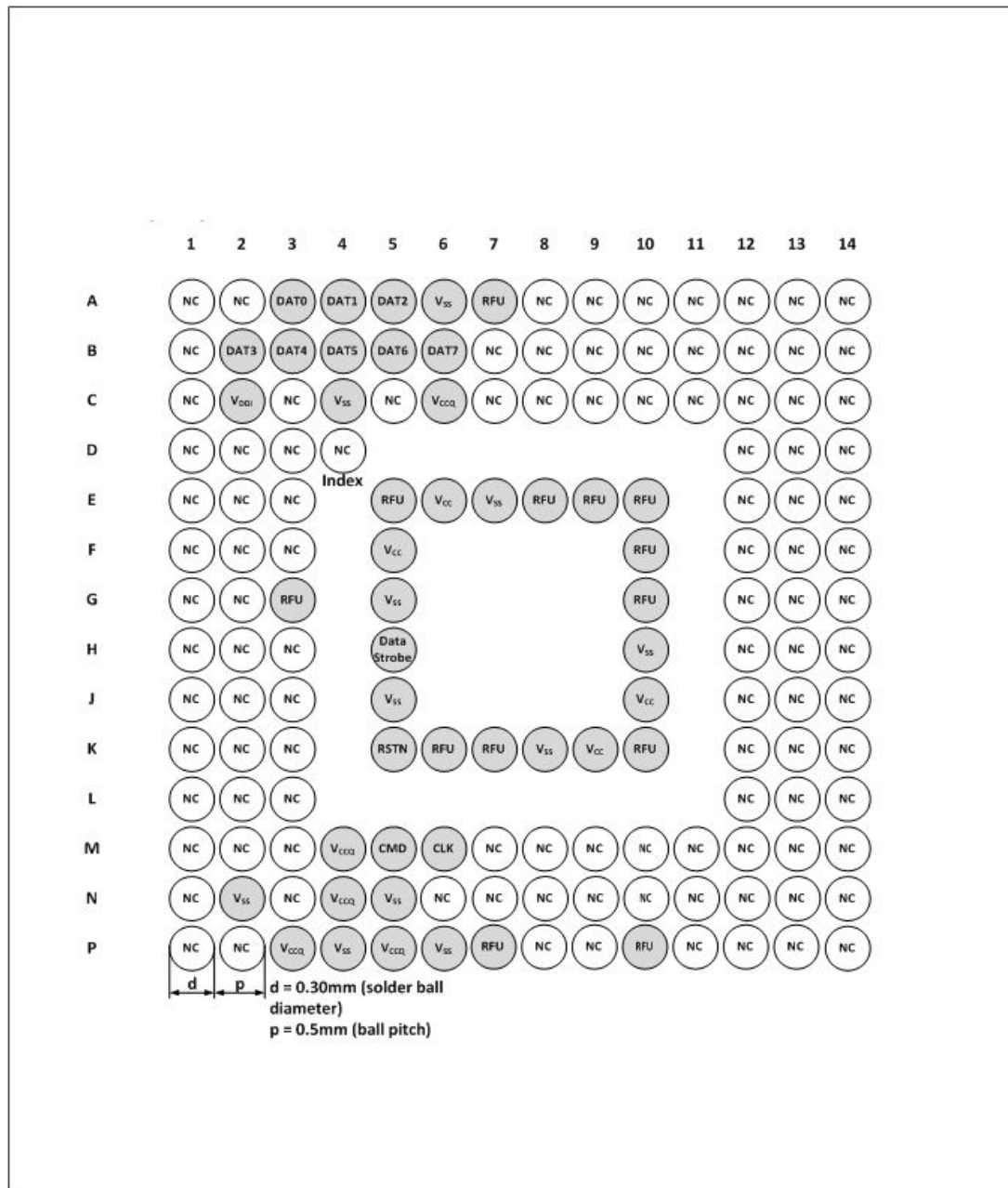
Figure 3. eMMC Package Ball Assignment
