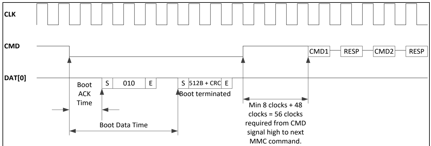
Figure 5. embedded MultiMediaCard state diagram (boot mode)
