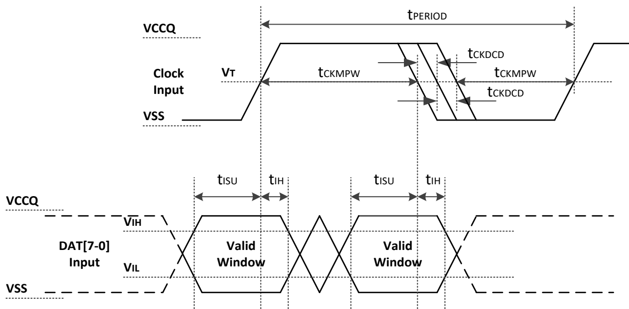
Figure 7. HS400 Device Input Timing Diagram
