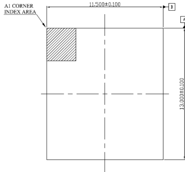
Figure 1-1. 11.5 x 13.0 x 1.0 (mm) Package Dimension
