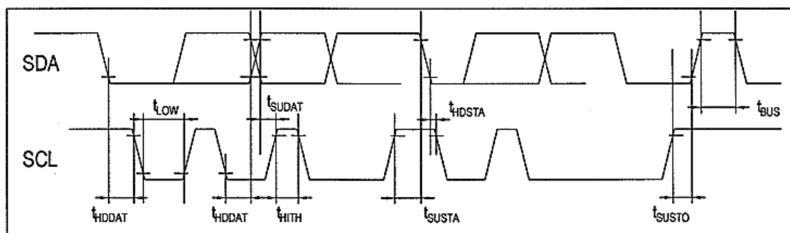
I 2 C INTERFACE TIMING DIAGRAM
