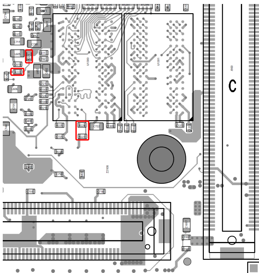
Figure 13: Pull-Up During Configuration (PUDC) and Power-on Reset Delay Override (PORSEL) Resistors - Assembly Drawing Bottom View (lower right part)
