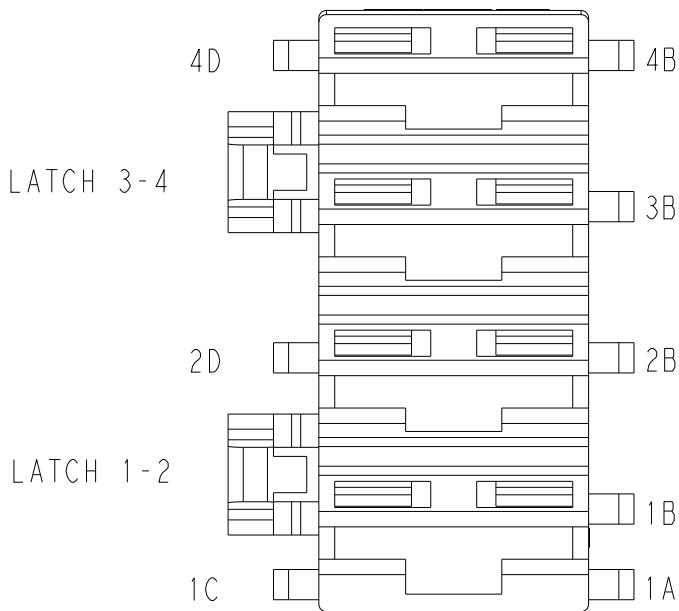
FRONT VIEW FOR CLARITY THIS VIEW SHOWS THE KEYING & POLARIZATION FEATURES ONLY
