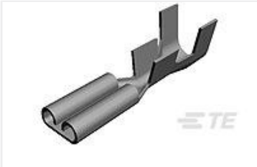
TE Part #41772 250 FASTON REC 22-18 AWG TPBR
