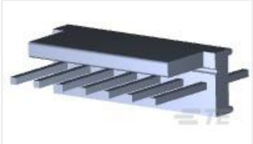
TE Part #3-641213-7 07P MTA100 HDR ASSY PO/ST LF
