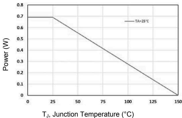
Figure 9. Power Dissipation
