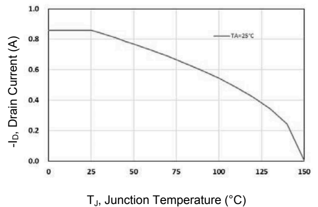
Figure 10. Drain Current
