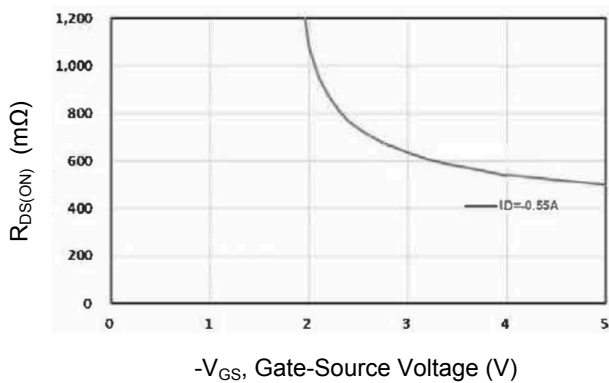
Figure 3. Power Dissipation
