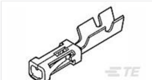
TE Part #166309-2 MOD-5 REC.CONTACT
