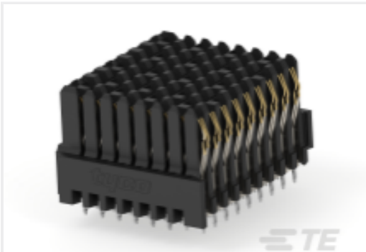
TE Part #2332817-2 Vert RCPT Left End Half Multigig RT 3
