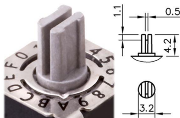
Slotted spindle
