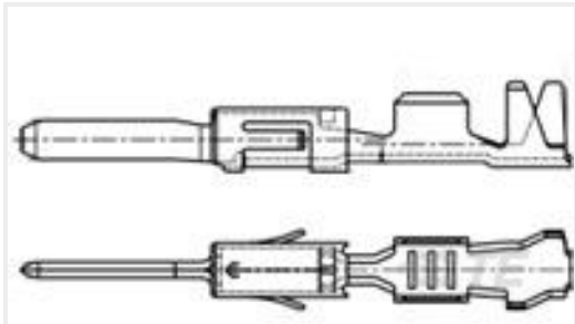
TE Part #963902-1 TAB A 1.6x0.6 CONTACT CS SWS Sn
