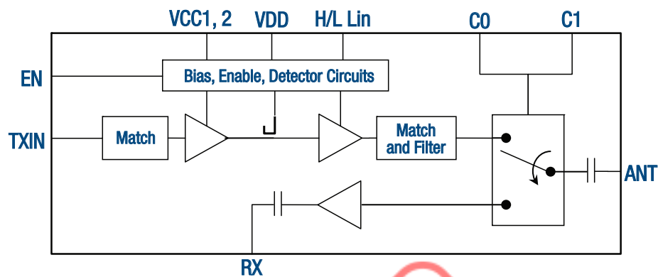
Figure 2. SE5012T Block Diagram
