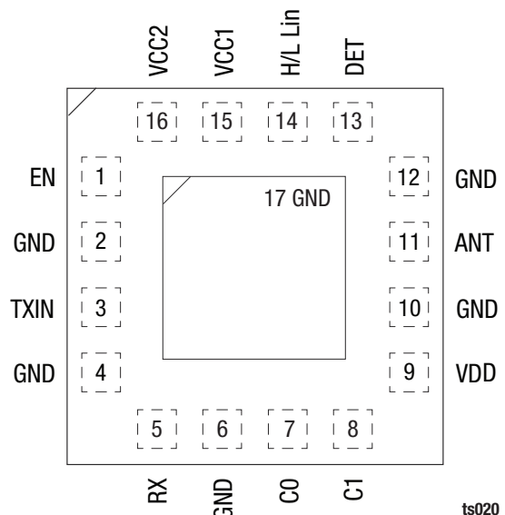
Figure 1. SE5012T Pinout – 16-Pin QFN (Top View)
