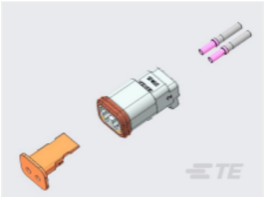
TE Part #DT06-2S-COMplete DT06-2S CON AND WEG
