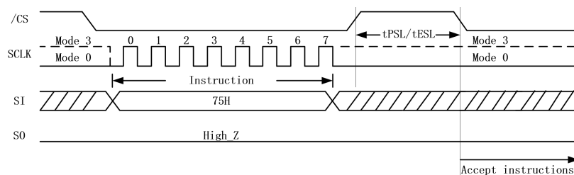
Figure 7.4.9. Program/Erase Suspend Instruction
