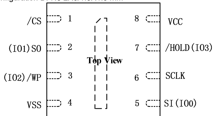
Figure 3a. Pin Configuration DFN8 2X3/1.5X1.5 mm
