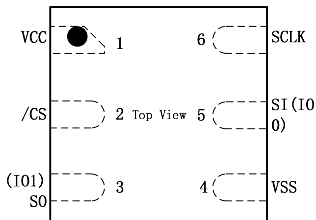
Figure 3b. Pin Configuration DFN6 1.2X1.2 mm
