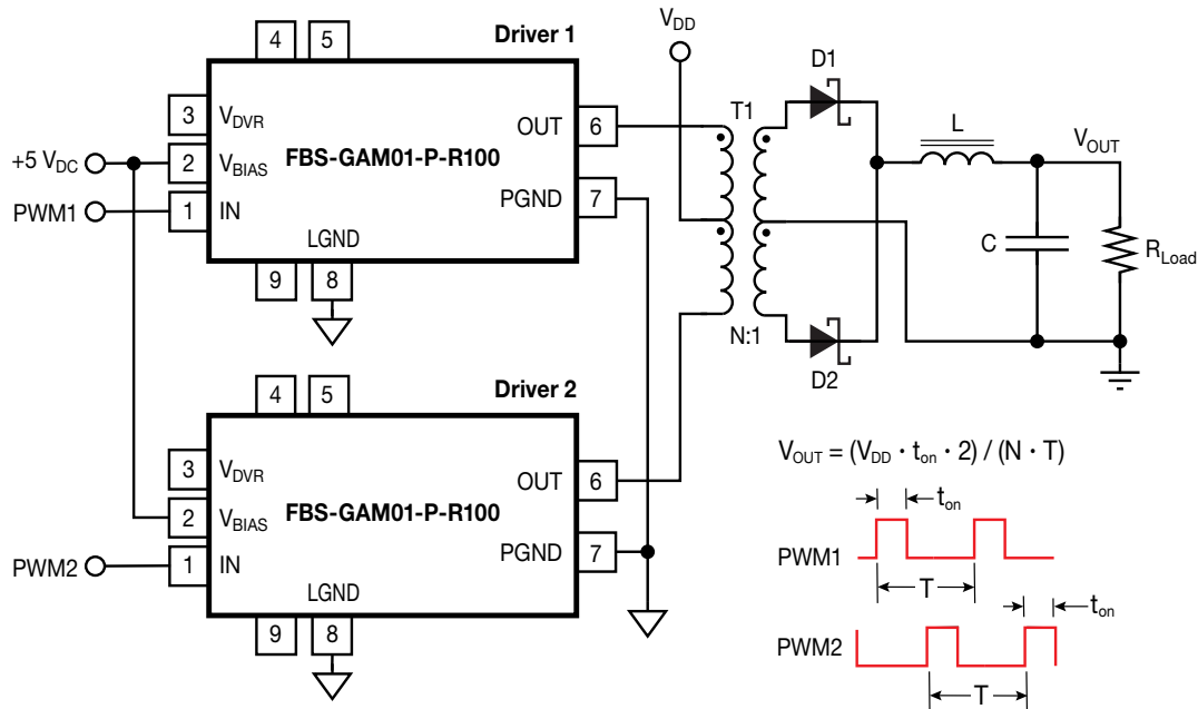
Figure 3. Push-Pull Converter
