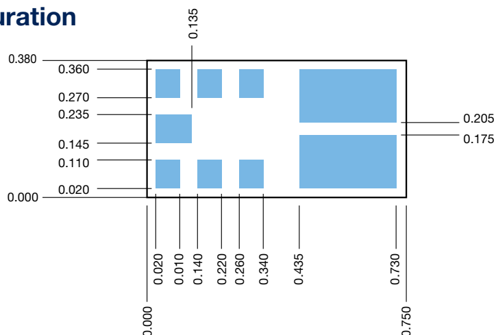
Figure 9. Recommended PCB Solder Pad Configuration (Bottom View)
