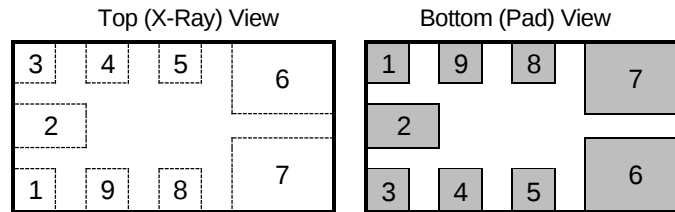
9 Pin Molded SMT Package with Pillar Pins
