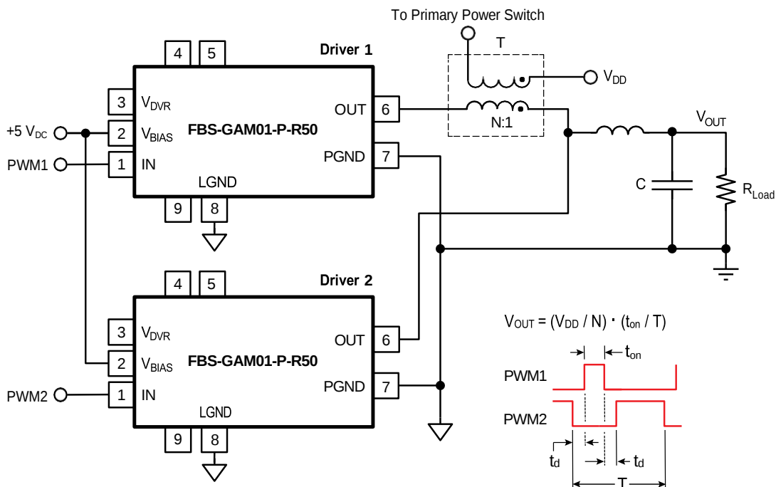
Figure 6. Synchronously-Rectified Forward Converter
