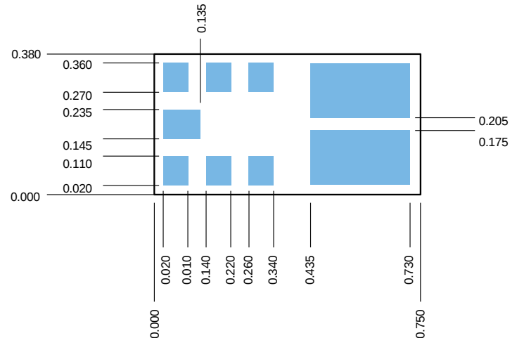
Figure 11. Recommended PCB Solder Pad Configuration (Bottom View)
