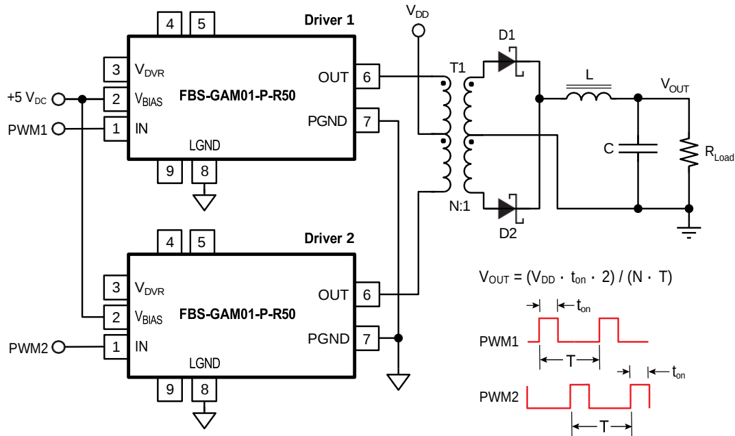
Figure 5. Push-Pull Converter
