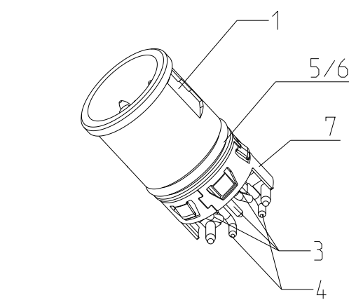
INDICATED PART-NO.225246-E
