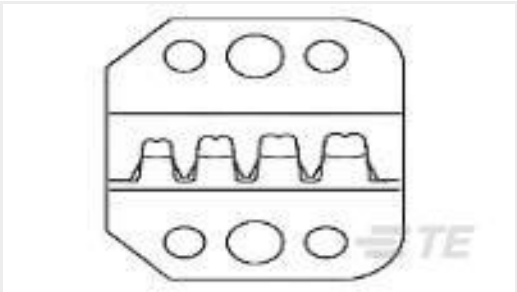
TE Part #58495-2 PROCRIPIER DIE ASSY MULTIMATE
