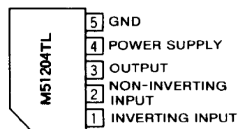
Outline 5P5T
