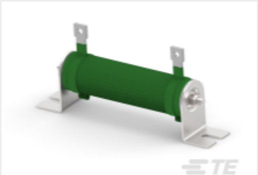
TE Part #CAT-C339-T2201 Wirewound Resistor: Mineral, 2.5 Kw
