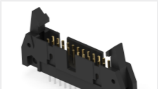
TE Part #2214643-5 A/L UNIV HDR 24P ACT PIN SHT L
