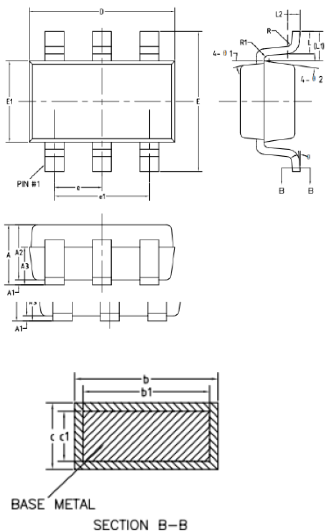
Figure 5. Outline Dimensions
