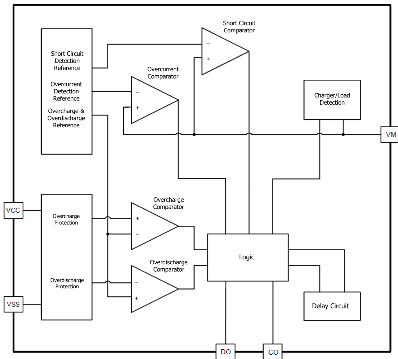
Figure 3. Block Diagram
