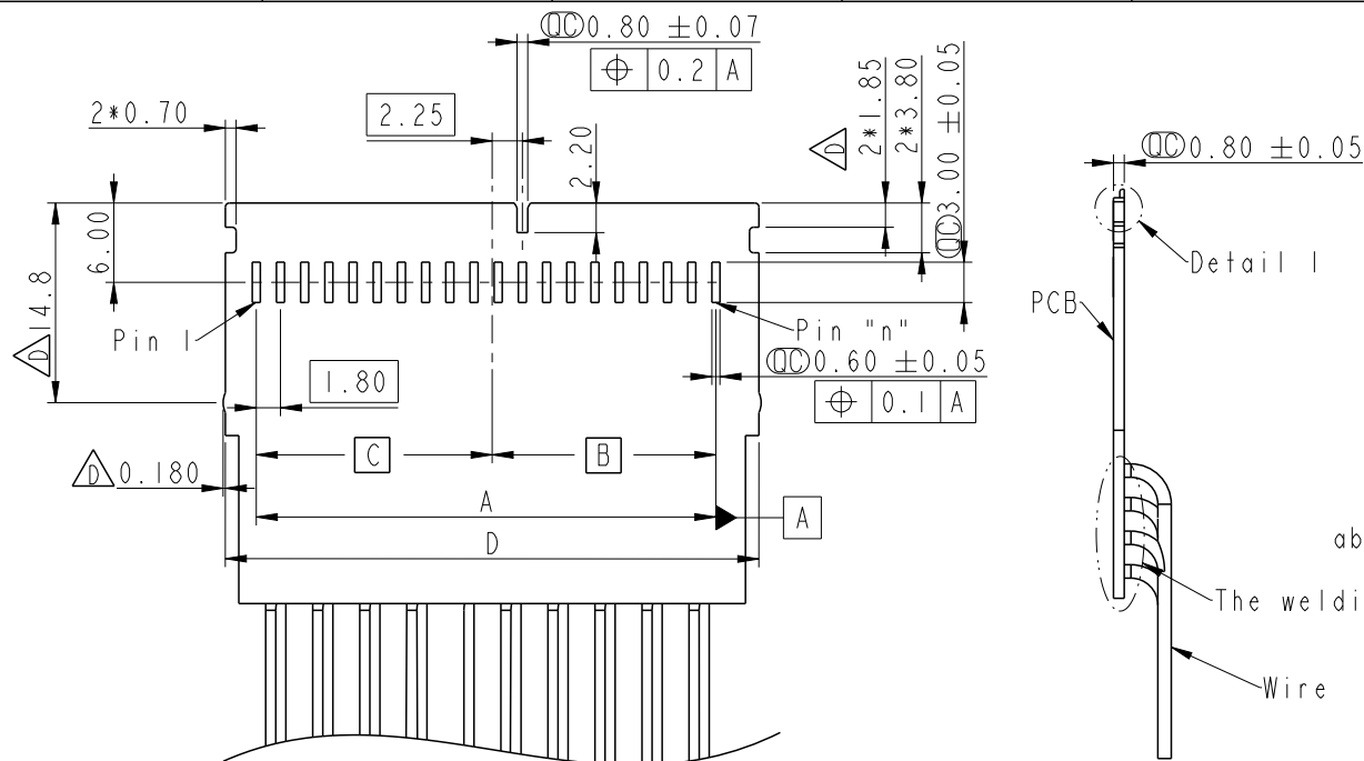
RECOMMENDED WTB LAYOUT
