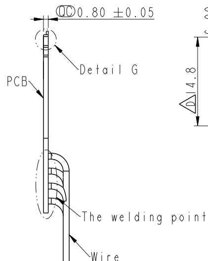
Recommend Optional 0.35 \pm 0.05 0.50 \triangle P Gold finger above flat surface Detail: G
