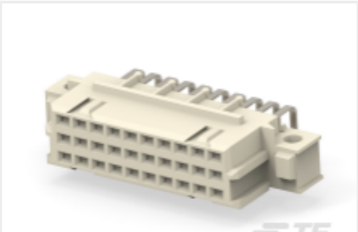
TE Part #254326-E STVR/3 30 FI ABC VV 7-03 TL * * 247 E 1
