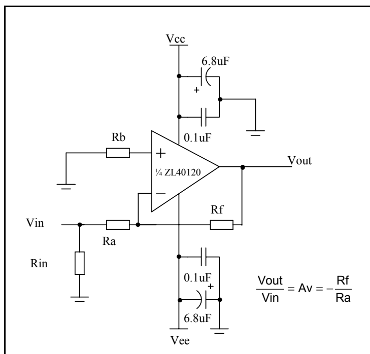
Figure 3 - Inverting Gain
