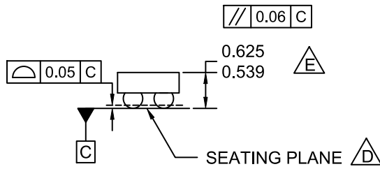
SIDE VIEWS
