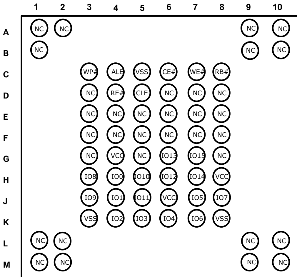
Figure 2.2 : 63-FBGA Contact, x16 Device, 11mm x 9mm
