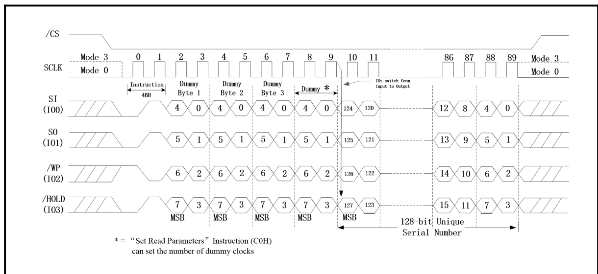
Figure 108. Read Unique ID Sequence Diagram (QPI Mode/3-Byte Address Mode)
