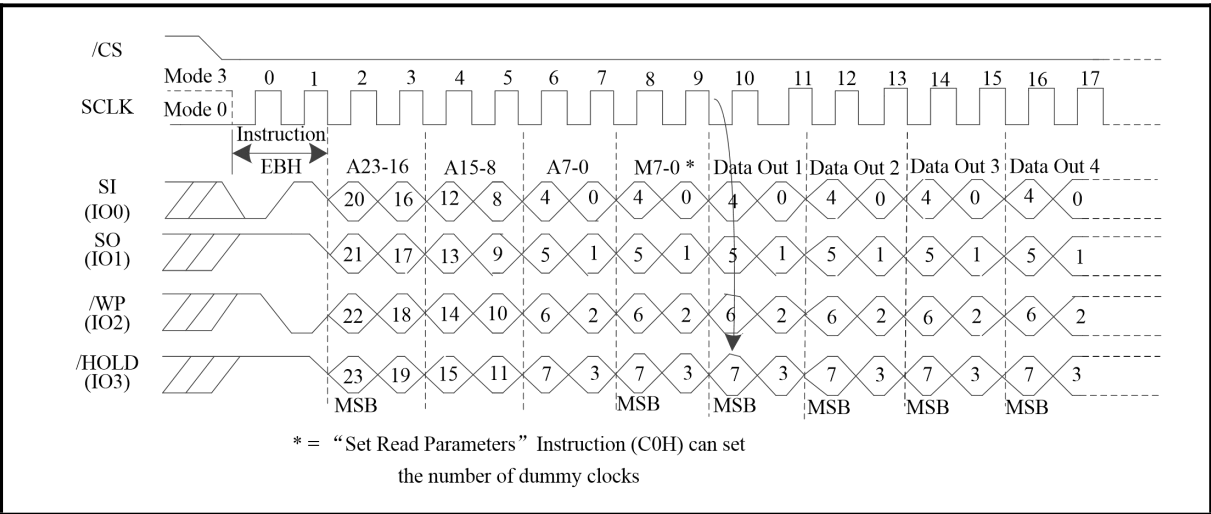
Figure 67. Quad I/O Fast Read Sequence Diagram (QPI Mode/3-Byte Address Mode; Initial instruction or previous (M5-4≠(1,0)))
