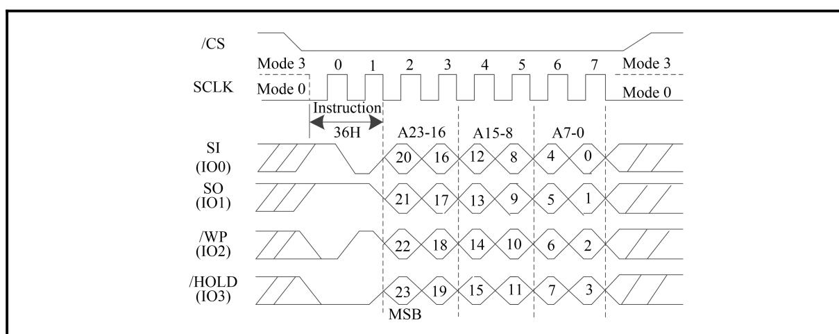
Figure 187. Dynamic Protection Block/Sector Lock (QPI Mode/3-Byte Address Mode)
