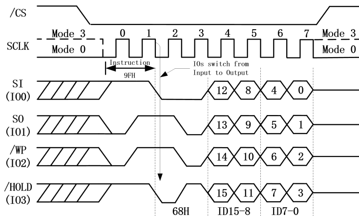
Figure 23.b. Read JEDEC ID Instruction (QPI Mode)
