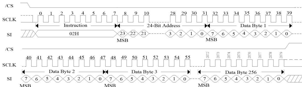
Figure 32.b. Page Program Instruction (QPI Mode)
