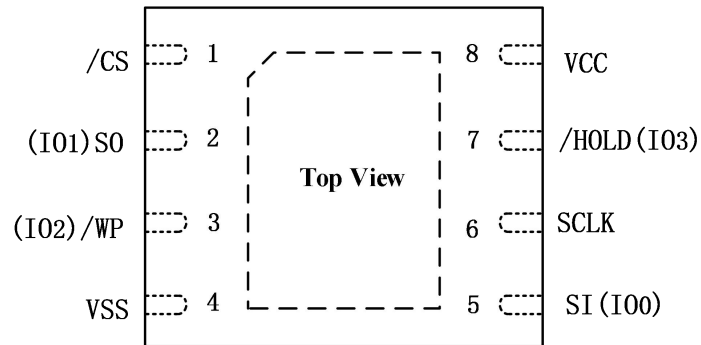
Figure 3.2. Pin Configuration USON 4X3mm
