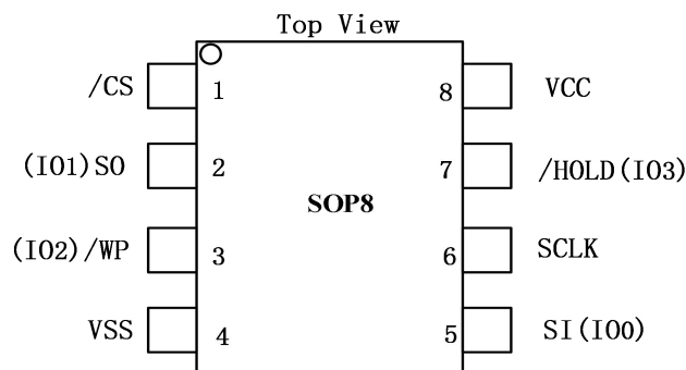
Figure 2. Pin Configuration SOP8
