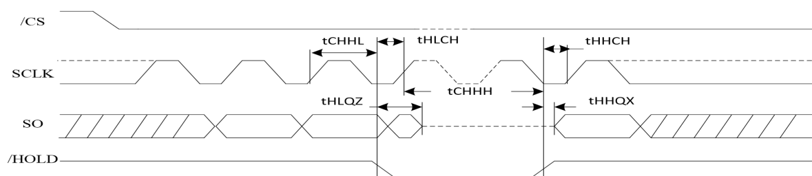
Figure 48. Hold Timing
