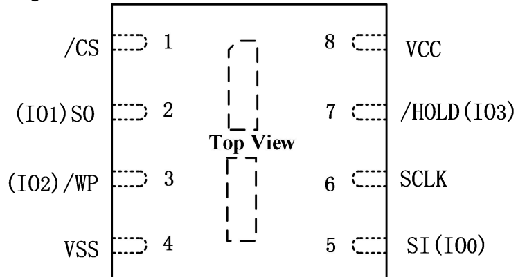
Figure 3.2. Pin Configuration USON 4X3mm
