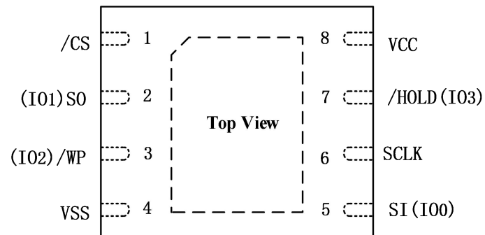
Figure 3.2. Pin Configuration USON 2X3mm
