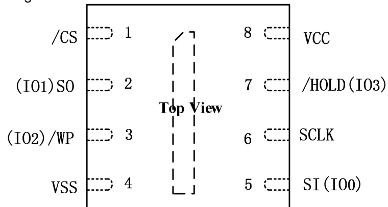
Figure 3.2. Pin Configuration USON 2X3mm
