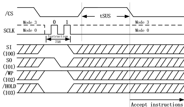
Figure 39.b. Program/Erase Suspend Instruction (QPI Mode)
