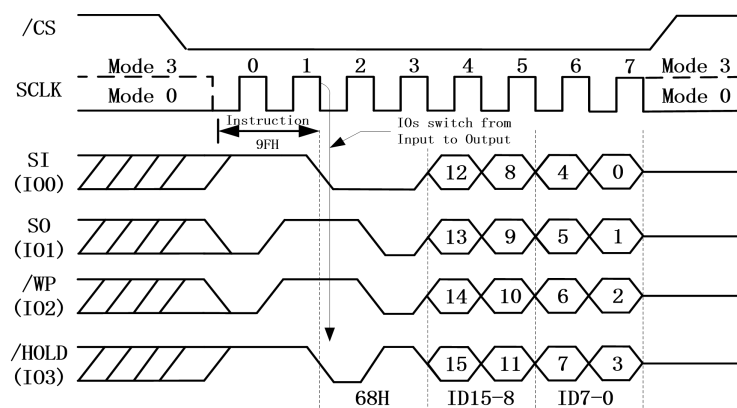
Figure 23.b. Read JEDEC ID Instruction (QPI Mode)
