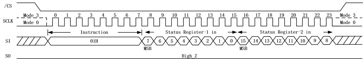
Figure 8.c. Write Status Register-1/2 Instruction (SPI Mode)
