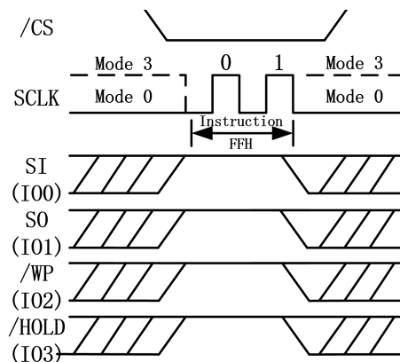
Figure 43. Exit QPI Instruction (QPI Mode only)
