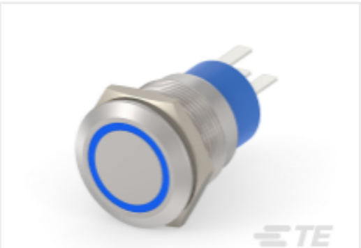
TE Part #1-2213764-9 AV19 SPM 3A FIX RING LED BLUE 24V
