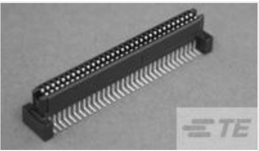
TE Part #1-120529-1 1FHR,64,50A/P,N,C,S11,12
