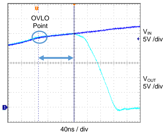
OVP Response Time ( V_{IN} = 20V to 90V Surge)
