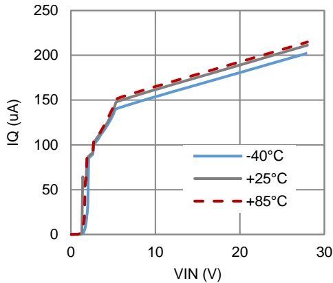
Supply Current vs VIN vs Temperature
