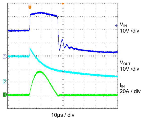
Surge Transient (90V)
