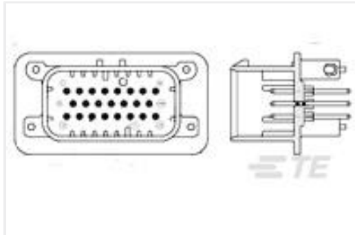
TE Part #776262-1 14POS,PIN DIA 1.3,HDR ASSY, 180DEG,COD 1
