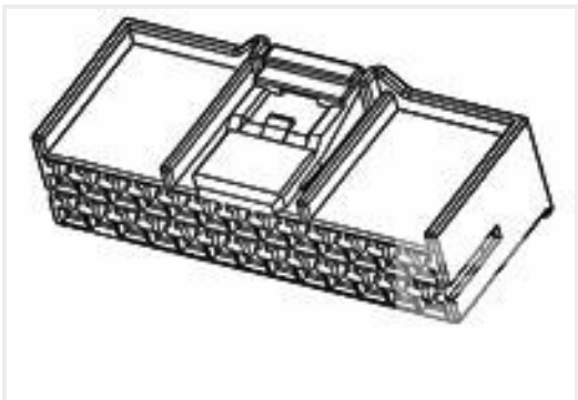
TE Part #936204-1 090III 18P PLUG ASSY
