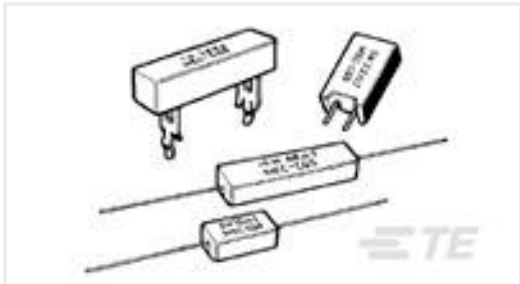
TE Part #1-1623779-4 SQB20 3R3 5% (WIRE)
