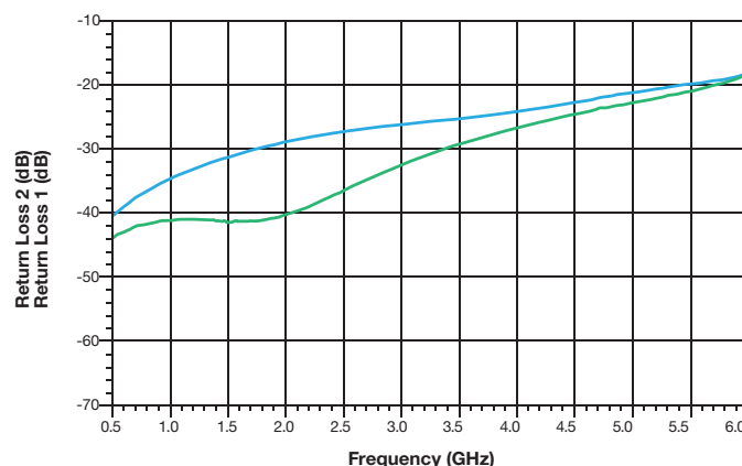
RF/RF Crossover – Return Loss
