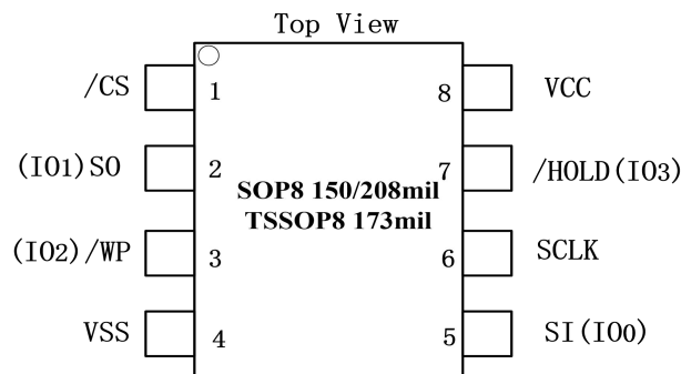
Figure 2. Pin Configuration SOP8 150/208mil, TSSOP8 173mil
