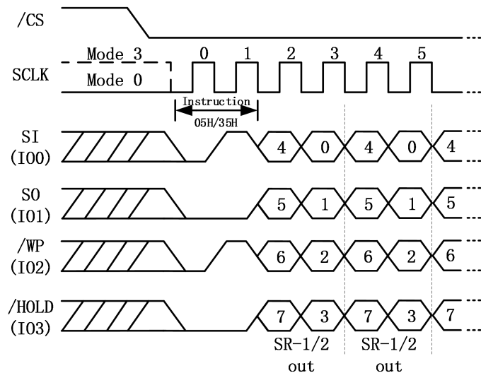
Figure 7.b. Read Status Register Sequence Diagram (QPI Mode)
