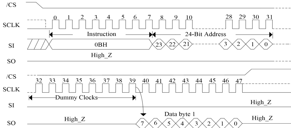
Figure 11.a. Fast Read Sequence Diagram (SPI Mode)
