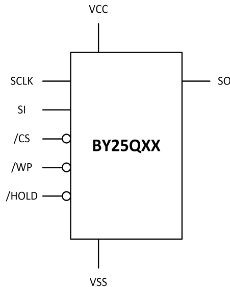
Figure 2. Pin Configuration SOP8 150/208mil, TSSOP8 173mil
