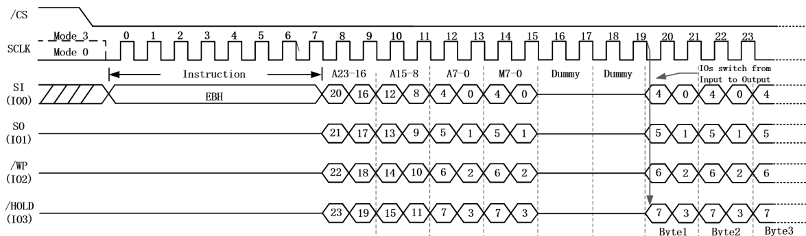
Figure 15.b. Quad I/O Fast Read Sequence Diagram (Previous command set (M5-4)=(1,0)), SPI mode)
