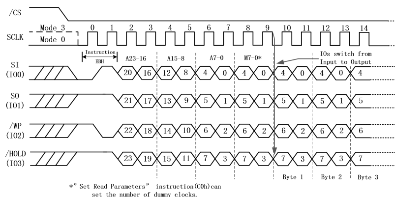
Figure 15.c. Quad I/O Fast Read Sequence Diagram (Initial instruction or previous (M5-4≠(1,0)) , QPI mode)
