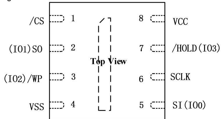
Figure 3. Pin Configuration USON8 2X3mm
