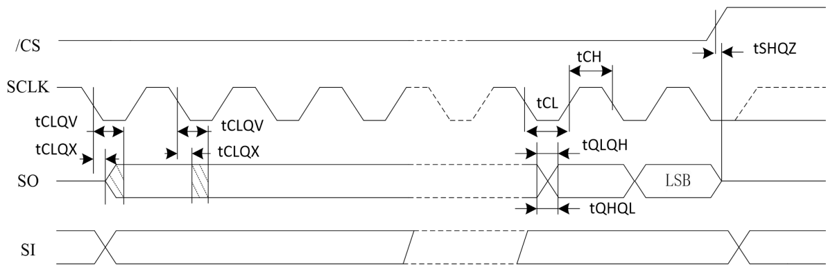
Figure 47. Output Timing
