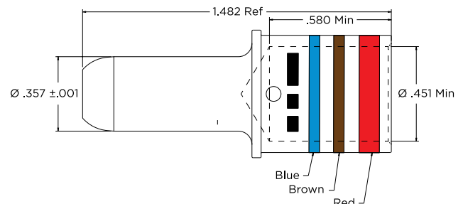
Part No. 0660-206-0082 Contact, Pin Size 0
