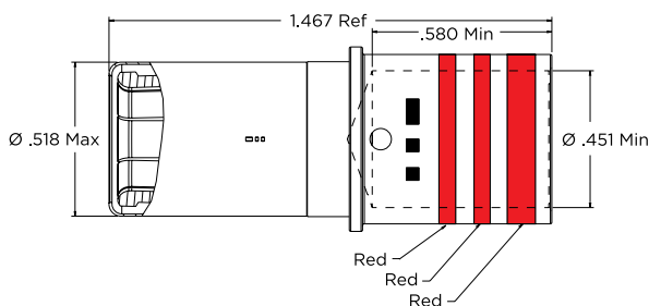
Part No. 0662-207-0082 Contact, Socket Size 0
