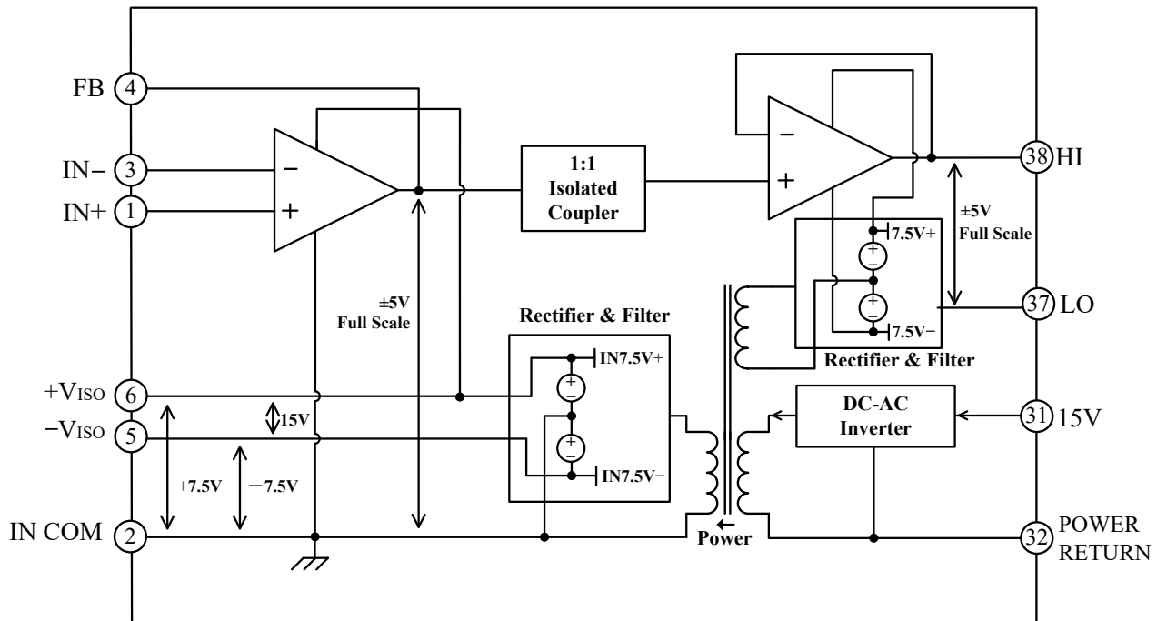
Figure 2. AD202JYATI Functional Block Diagram
