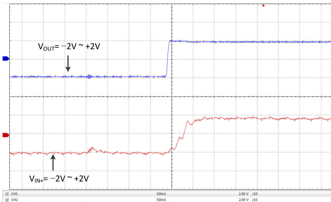
Figure 4. Rise time @ V_{IN+} = -2V \sim +2V
