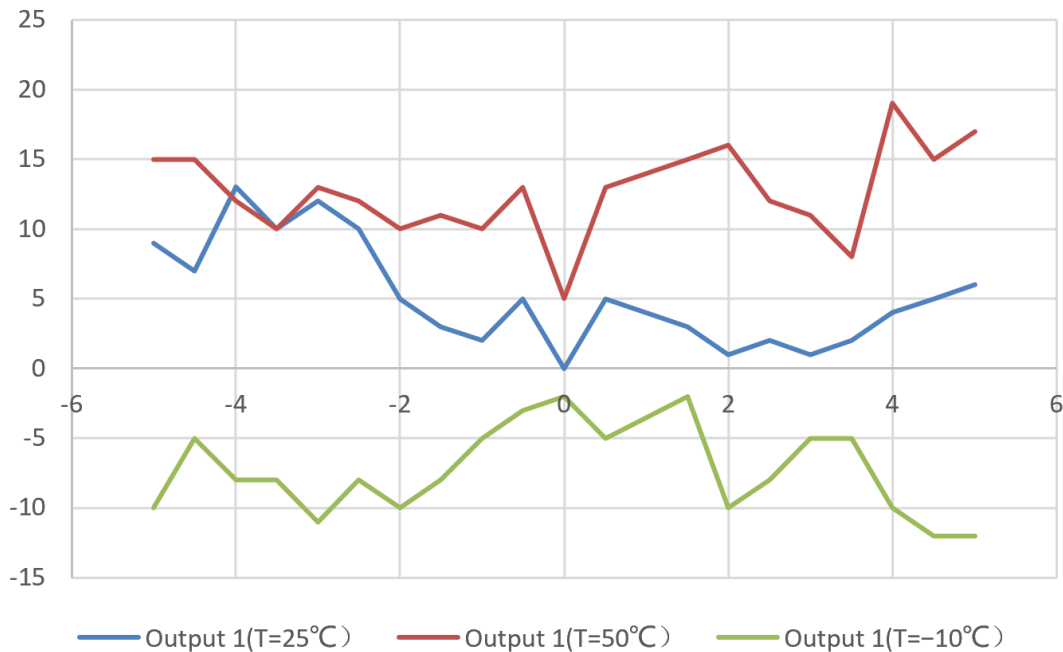
Figure 9. Nonlinearity
