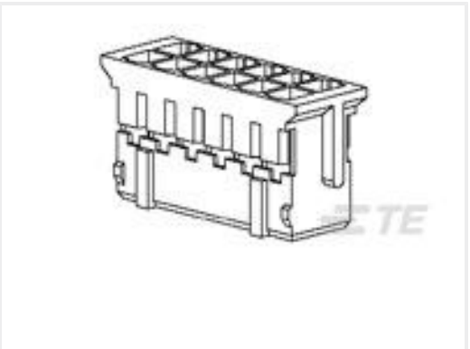
TE Part #1-1470107-0 2.0MM PITCH CRIMP HOUSING 10P
