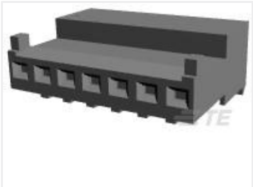
TE Part #3-643814-7 07P MTA100 CONN ASSY POL RIB
