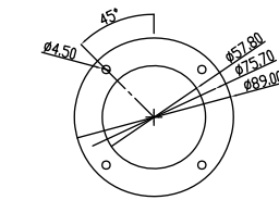
SS2-50P Power Inlet Seal Pad
